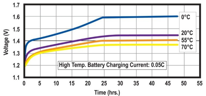
Trickle Charge
